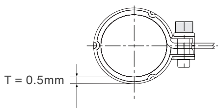
Outer jacket with clamps
